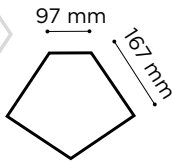
SMALL PENTAGON - MATERIAL \neq 6 mm
